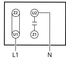
Driftkondensator, (motsols rotation)
